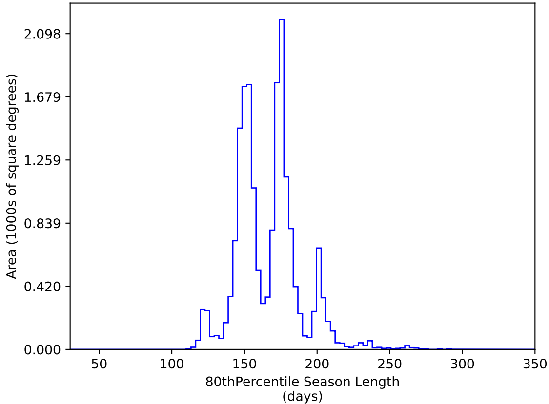
ddf_acor_sf10_lsf15_lsr10_v3.4_10yrs WFD y band: 80thPercentile Season Length
