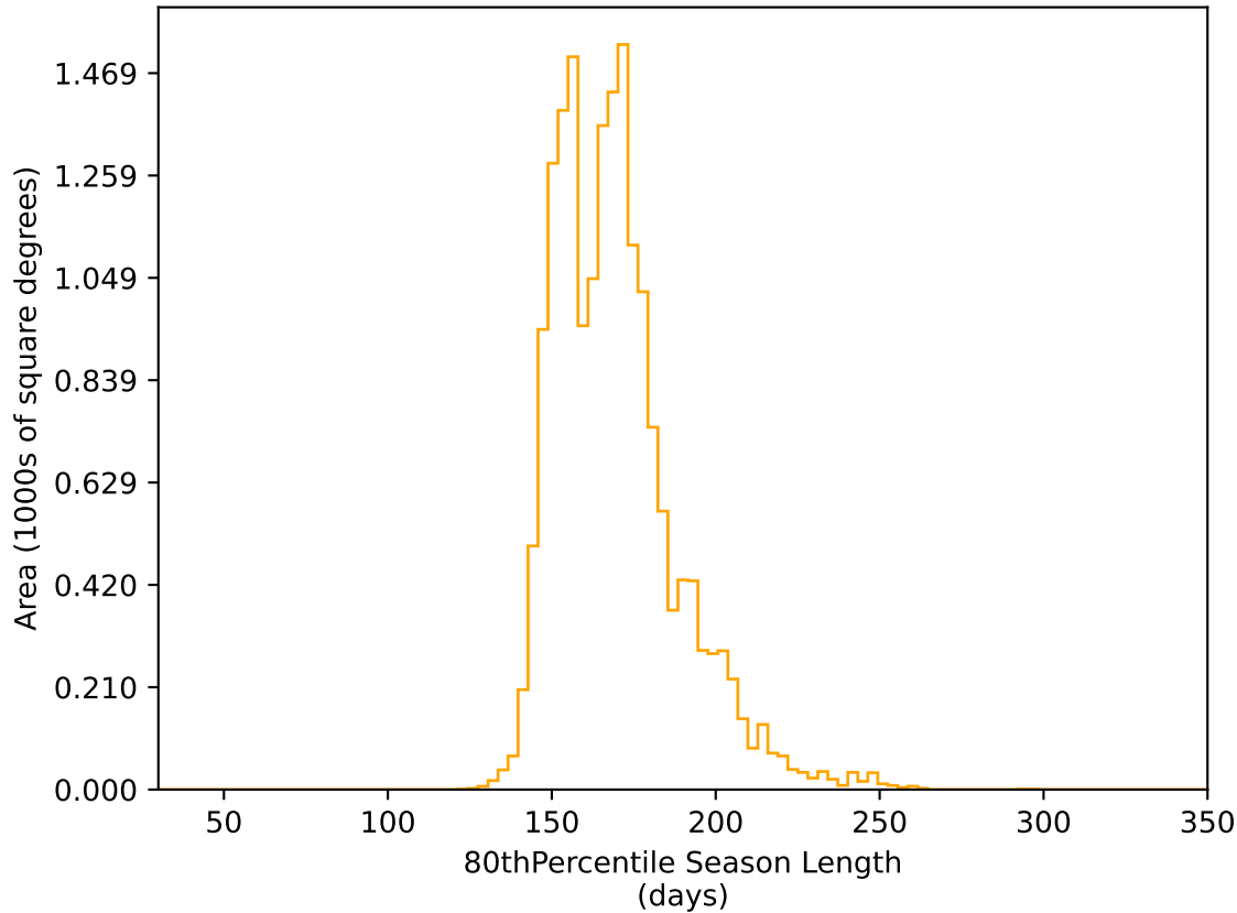
ddf_acor_sf10_lsf15_lsr10_v3.4_10yrs WFD r band: 80thPercentile Season Length
