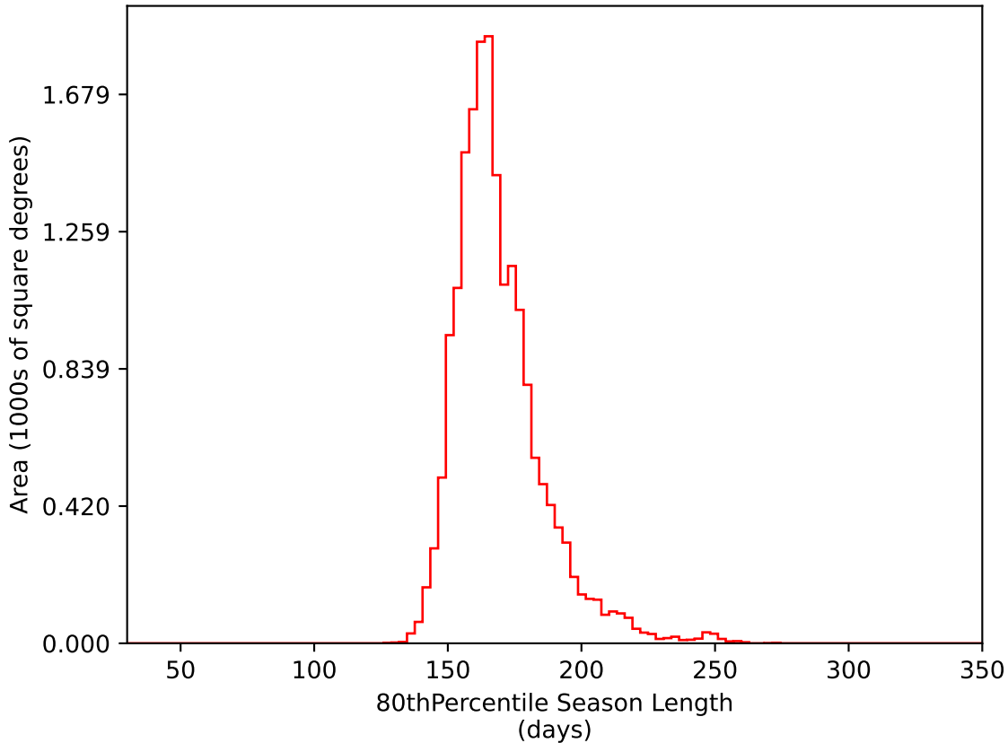
ddf_acor_sf10_lsf15_lsr10_v3.4_10yrs WFD i band: 80thPercentile Season Length
