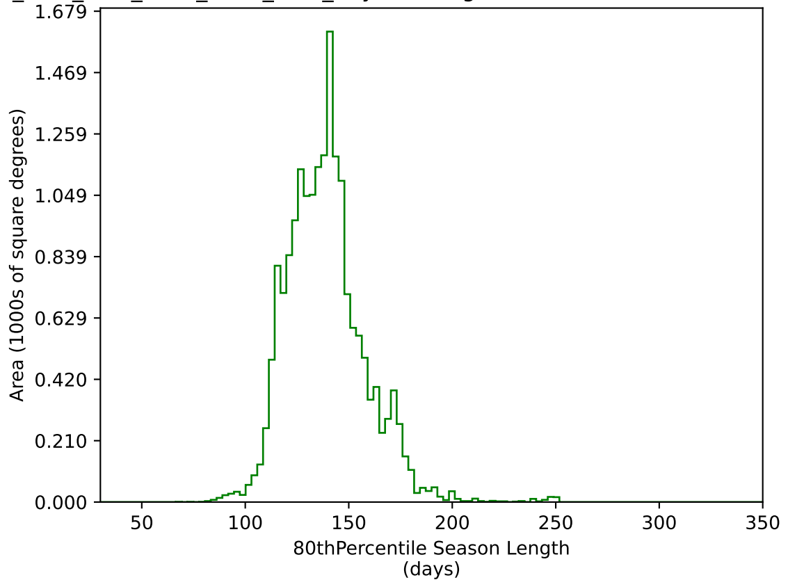
ddf_acor_sf10_lsf15_lsr10_v3.4_10yrs WFD g band: 80thPercentile Season Length
