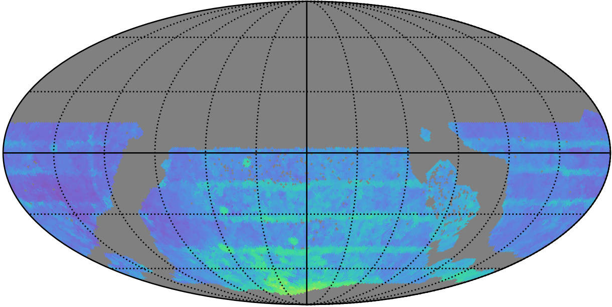
ddf_acor_sf10_lsf15_lsr10_v3.4_10yrs WFD all bands: 80thPercentile Season Length
