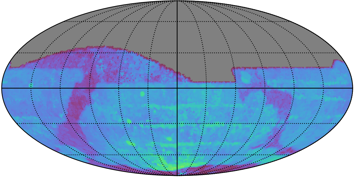
ddf_acor_sf10_lsf15_lsr10_v3.4_10yrs All sky z band: 80thPercentile Season Length
