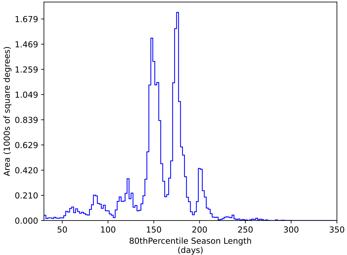
ddf_acor_sf10_ls15_lsr10_v3.4_10yrs All sky y band: 80thPercentile Season Length
