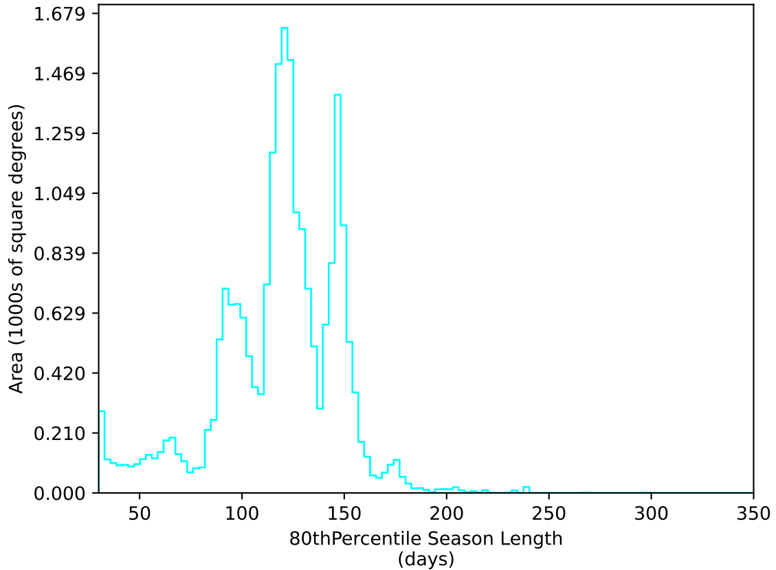
ddf_acor_sf10_lsf15_lsr10_v3.4_10yrs All sky u band: 80thPercentile Season Length
