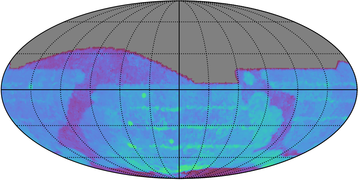
ddf_acor_sf10_lsf15_lsr10_v3.4_10yrs All sky r band: 80thPercentile Season Length
