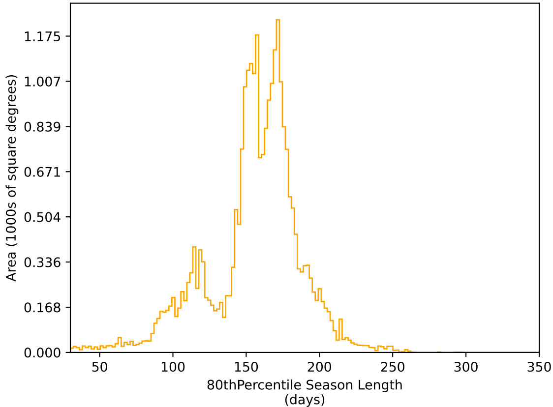
ddf_acor_sf10_lsf15_lsr10_v3.4_10yrs All sky r band: 80thPercentile Season Length
