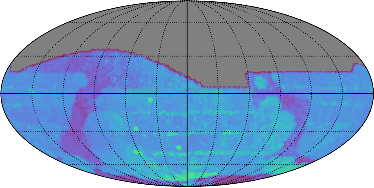
ddf_acor_sf10_lsf15_lsr10_v3.4_10yrs All sky i band: 80thPercentile Season Length
