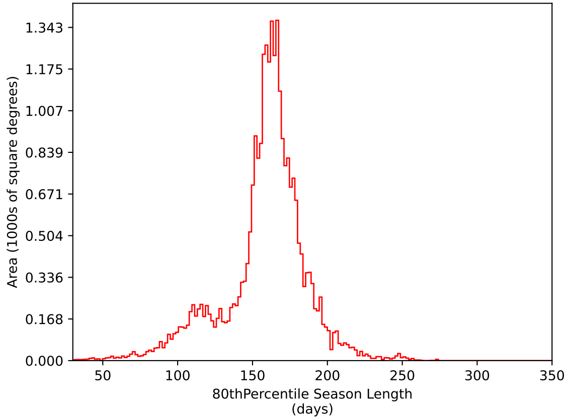
ddf_acor_sf10_lsf15_lsr10_v3.4_10yrs All sky i band: 80thPercentile Season Length
