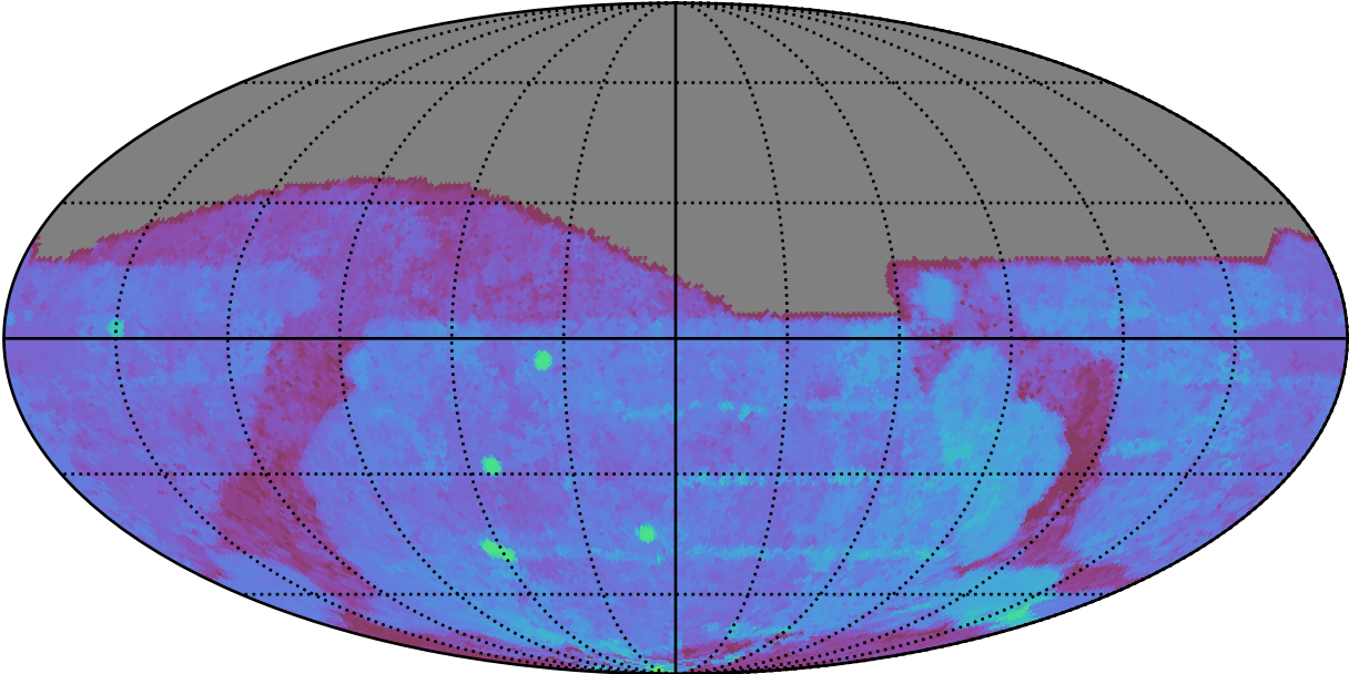
ddf_acor_sf10_lsf15_lsr10_v3.4_10yrs All sky g band: 80thPercentile Season Length
