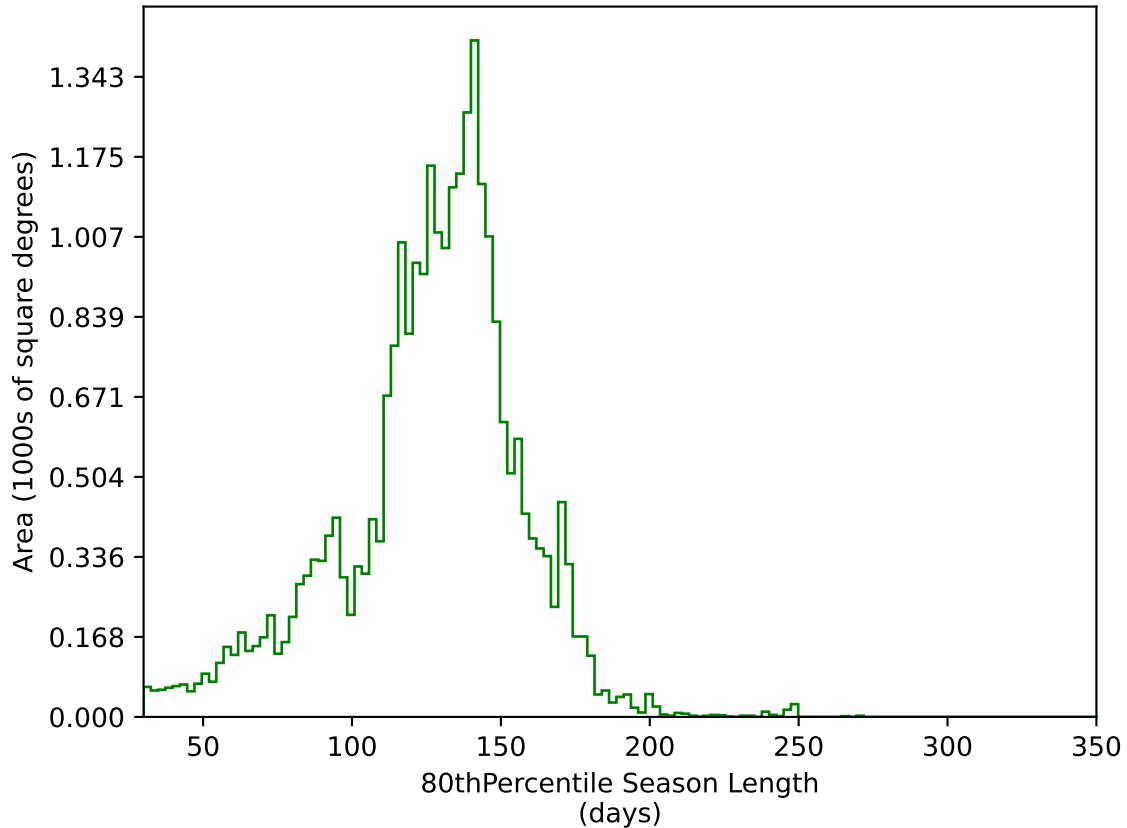
ddf_acor_sf10_ls15_lsr10_v3.4_10yrs All sky g band: 80thPercentile Season Length
