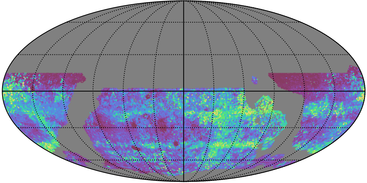
ddf_acor_sf10_lsf15_lsr10_v3.4_10yrs WFD zy bands: 75th Percentile Intranight Timespan
