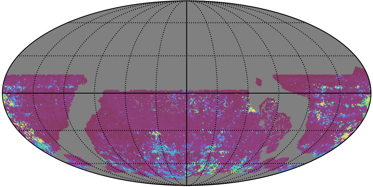
ddf_acor_sf10_lsf15_lsr10_v3.4_10yrs WFD z band: 75th Percentile Intranight Timespan
