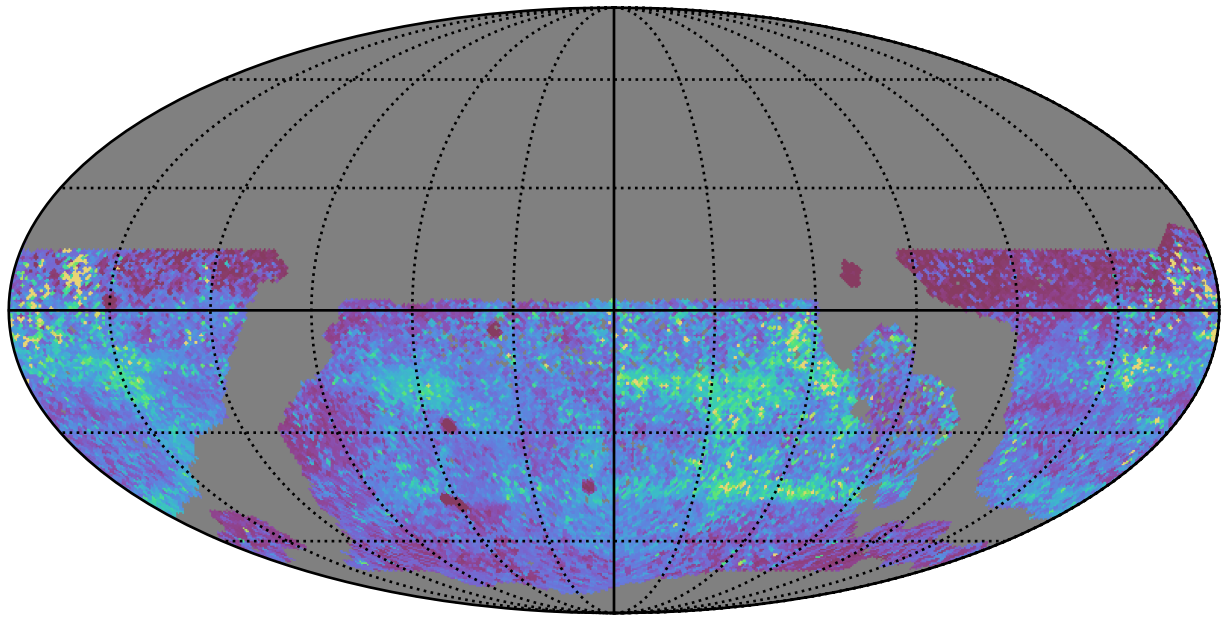
ddf_acor_sf10_lsf15_lsr10_v3.4_10yrs WFD y band: 75th Percentile Intranight Timespan
