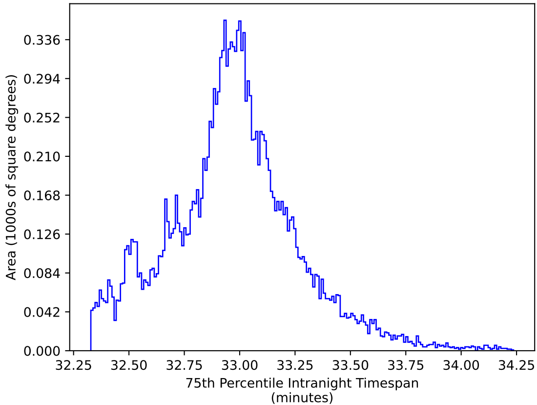
ddf_acor_sf10_lsf15_lsr10_v3.4_10yrs WFD y band: 75th Percentile Intranight Timespan
