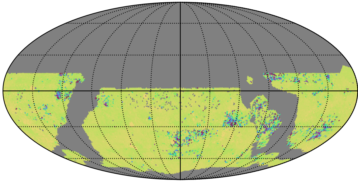
ddf_acor_sf10_lsf15_lsr10_v3.4_10yrs WFD ug bands: 75th Percentile Intranight Timespan
