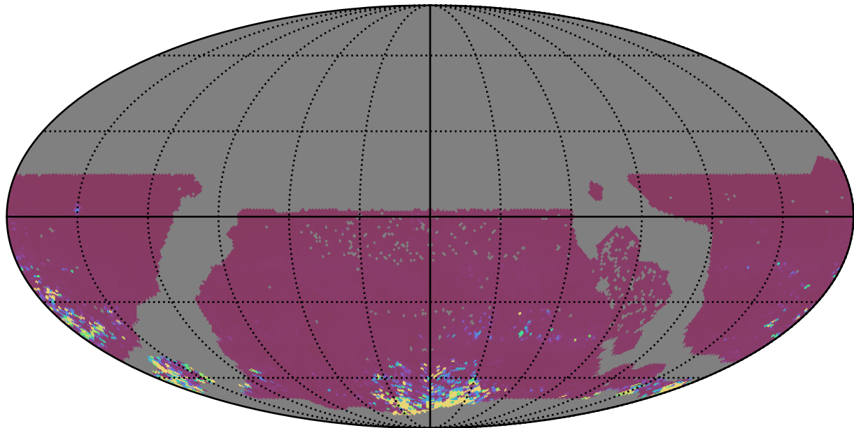
ddf_acor_sf10_lsf15_lsr10_v3.4_10yrs WFD ri bands: 75th Percentile Intranight Timespan
