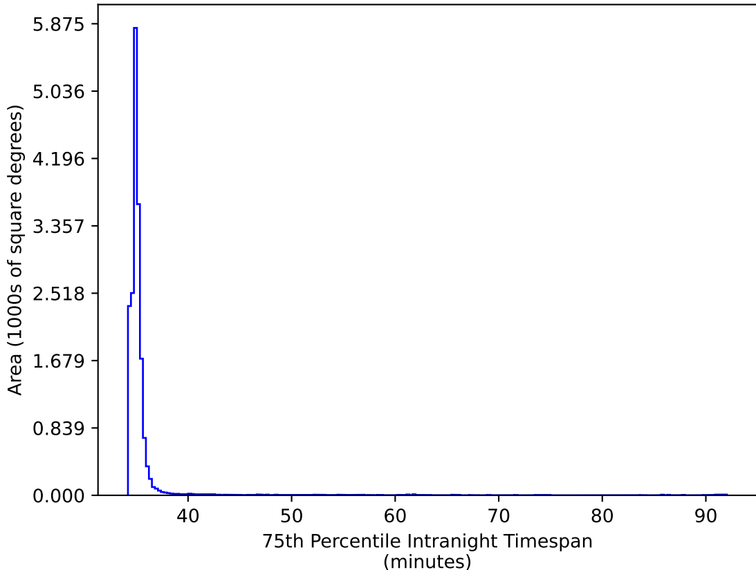
ddf_acor_sf10_lsf15_lsr10_v3.4_10yrs WFD ri bands: 75th Percentile Intranight Timespan
