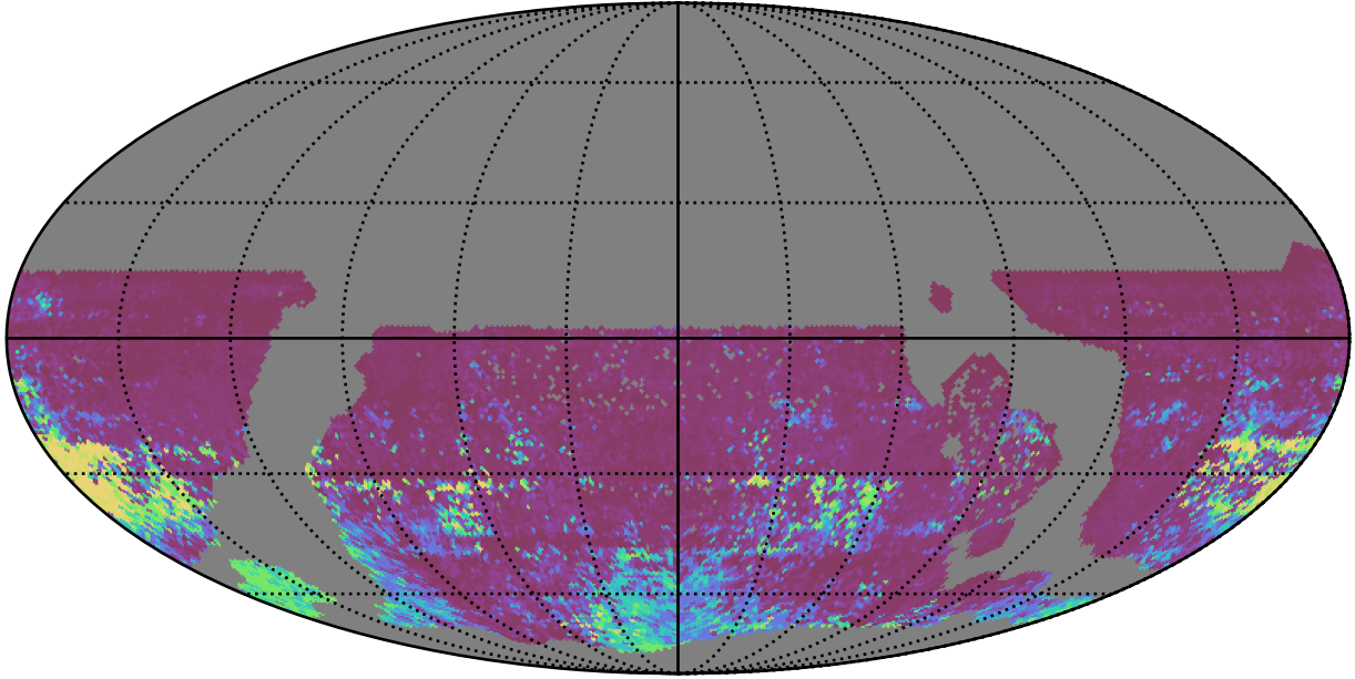
ddf_acor_sf10_ls15_lsr10_v3.4_10yrs WFD r band: 75th Percentile Intranight Timespan
