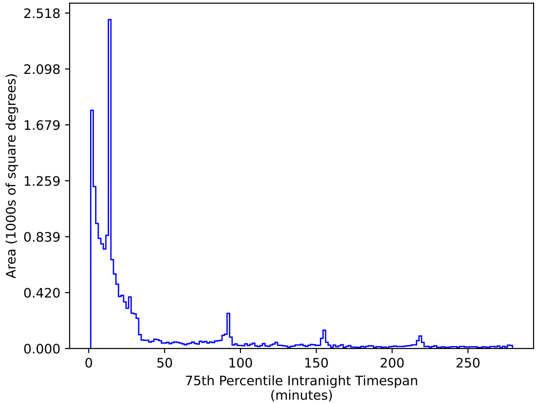
ddf_acor_sf10_ls15_lsr10_v3.4_10yrs WFD r band: 75th Percentile Intranight Timespan
