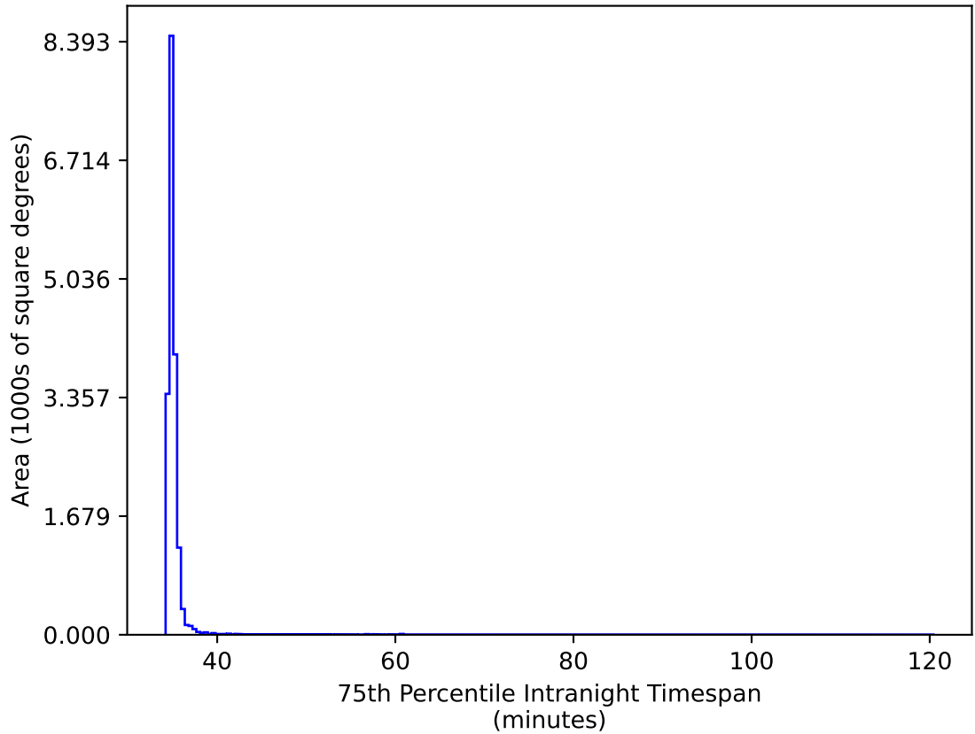
ddf_acor_sf10_lsf15_lsr10_v3.4_10yrs WFD gr bands: 75th Percentile Intranight Timespan
