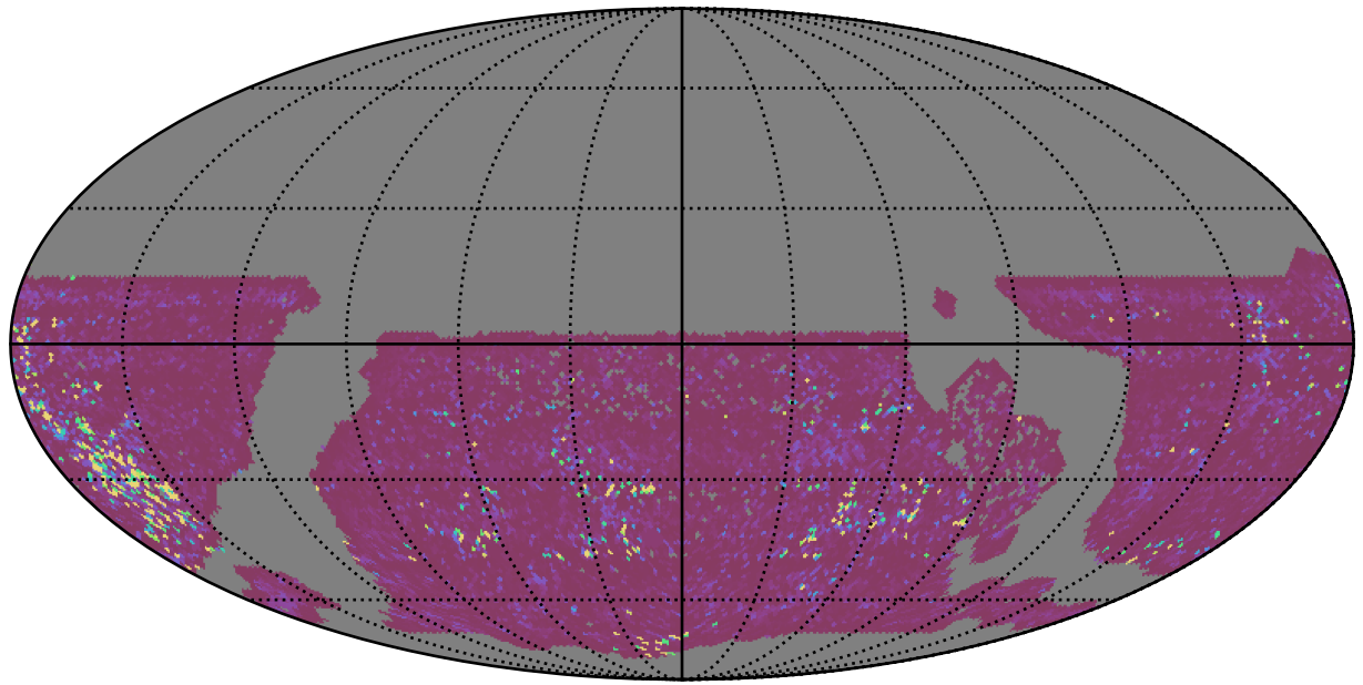
ddf_acor_sf10_lsf15_lsr10_v3.4_10yrs WFD g band: 75th Percentile Intranight Timespan
