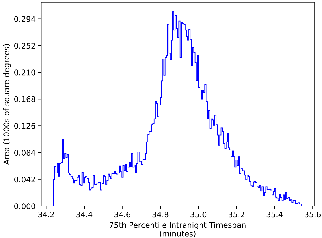
ddf_acor_sf10_ls15_lsr10_v3.4_10yrs WFD all bands: 75th Percentile Intranight Timespan
