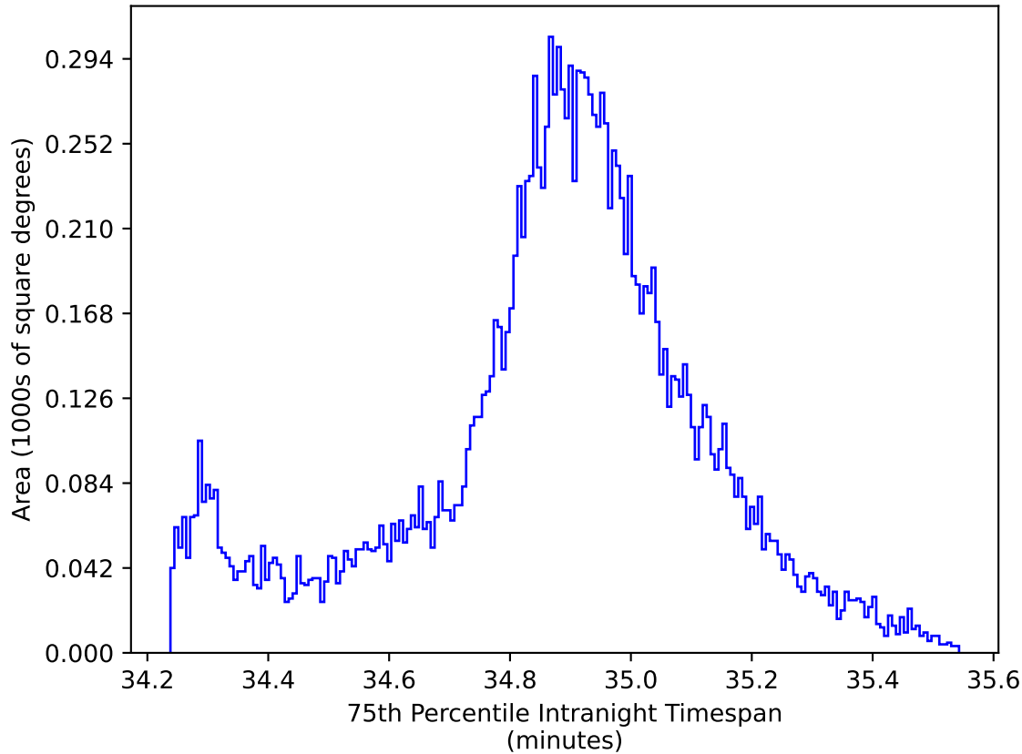
ddf_acor_sf10_lsf15_lsr10_v3.4_10yrs WFD: 75th Percentile Intranight Timespan
