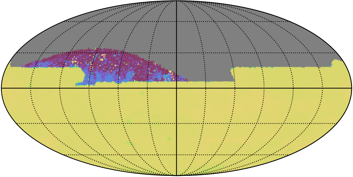
ddf_acor_sf10_lsf15_lsr10_v3.4_10yrs All sky zy bands: 75th Percentile Intranight Timespan
