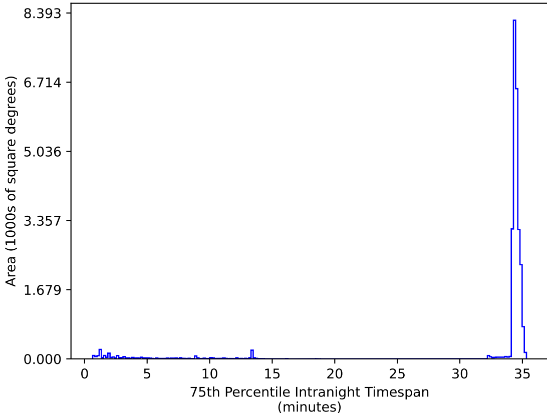
ddf_acor_sf10_lsf15_lsr10_v3.4_10yrs All sky zy bands: 75th Percentile Intranight Timespan
