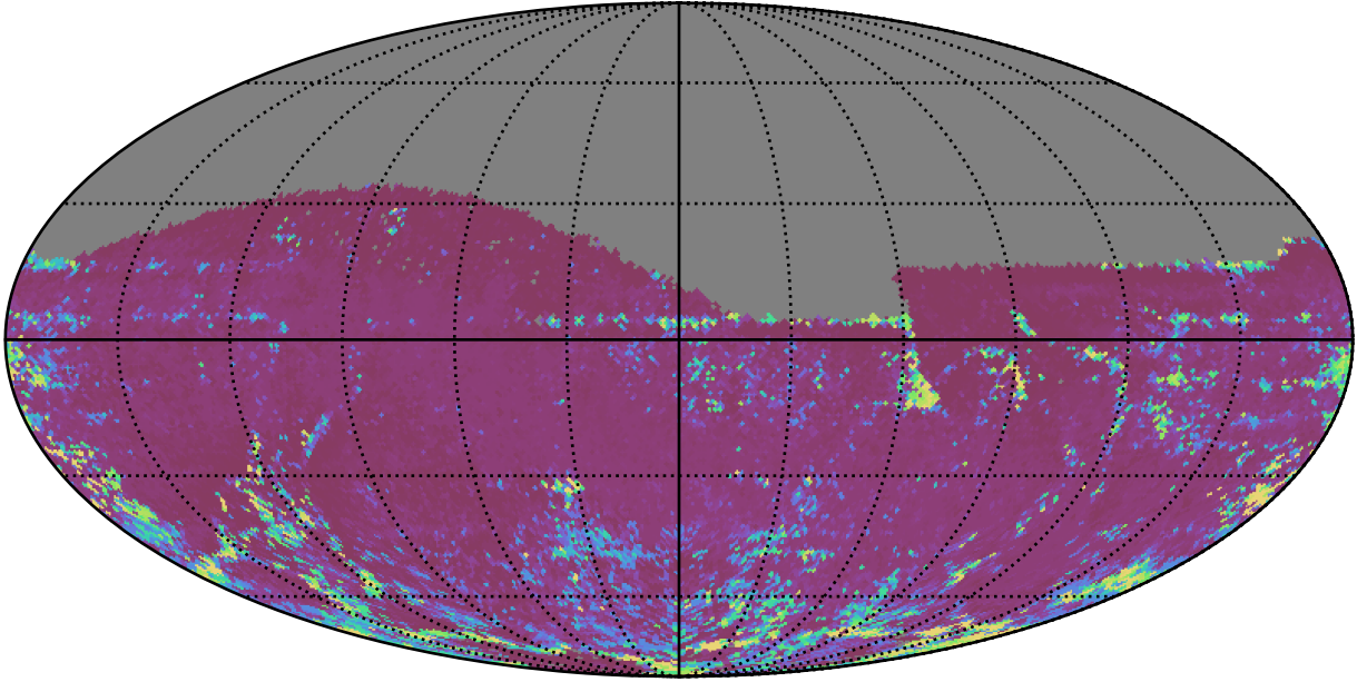
ddf_acor_sf10_lsf15_lsr10_v3.4_10yrs All sky z band: 75th Percentile Intranight Timespan
