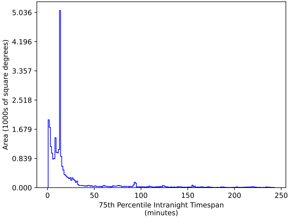
ddf_acor_sf10_lsf15_lsr10_v3.4_10yrs All sky z band: 75th Percentile Intranight Timespan
