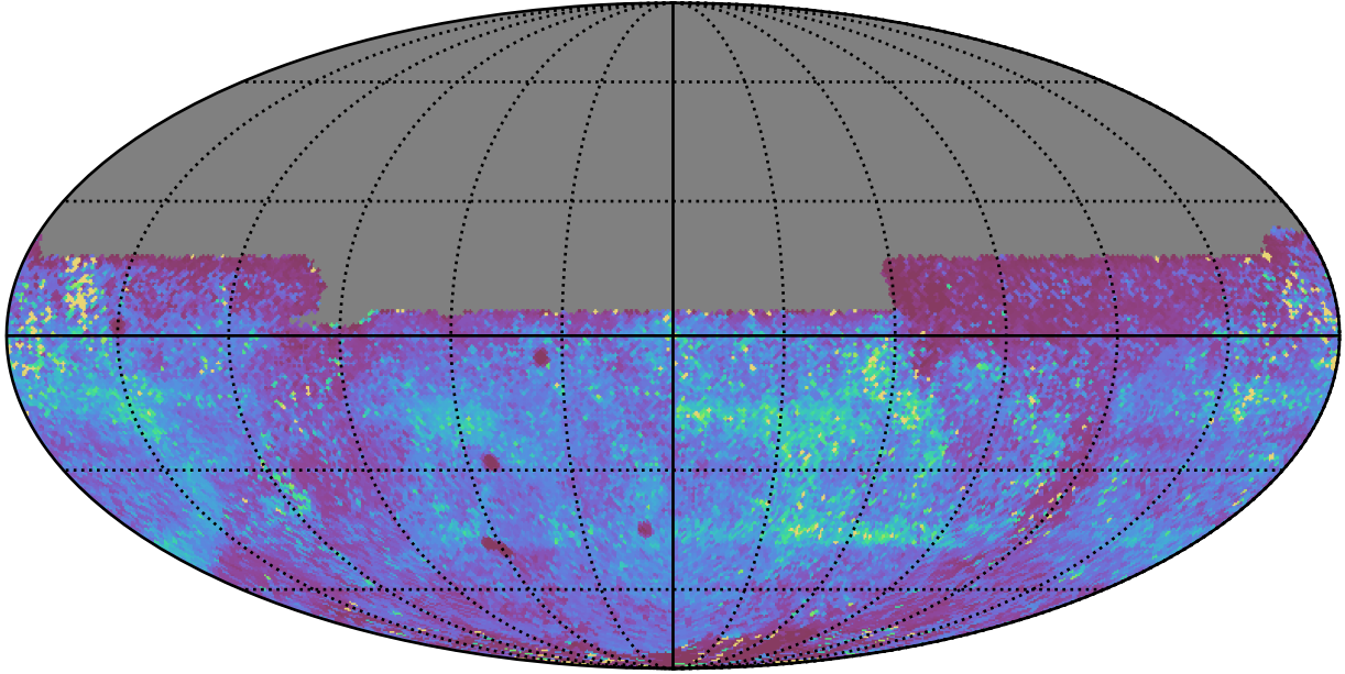
ddf_acor_sf10_lsf15_lsr10_v3.4_10yrs All sky y band: 75th Percentile Intranight Timespan
