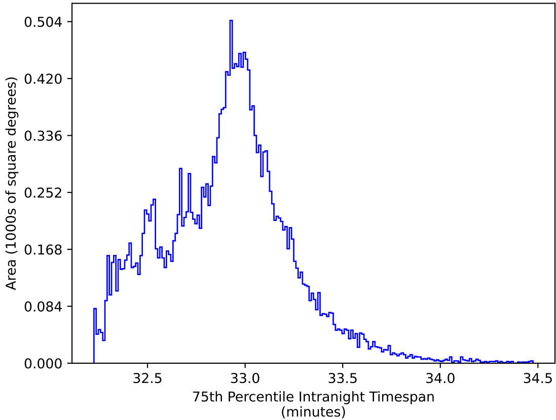
ddf_acor_sf10_ls15_lsr10_v3.4_10yrs All sky y band: 75th Percentile Intranight Timespan
