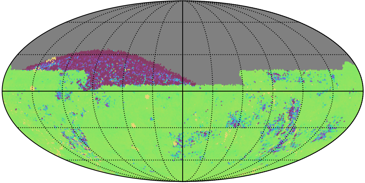
ddf_acor_sf10_lsf15_lsr10_v3.4_10yrs All sky ug bands: 75th Percentile Intranight Timespan
