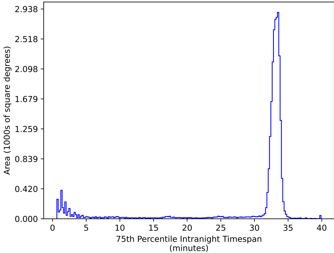
ddf_acor_sf10_lsf15_lsr10_v3.4_10yrs All sky ug bands: 75th Percentile Intranight Timespan
