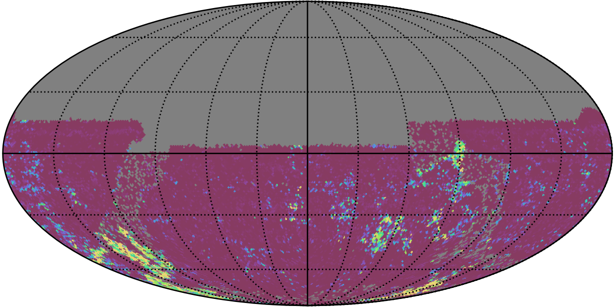
ddf_acor_sf10_lsf15_lsr10_v3.4_10yrs All sky u band: 75th Percentile Intranight Timespan
