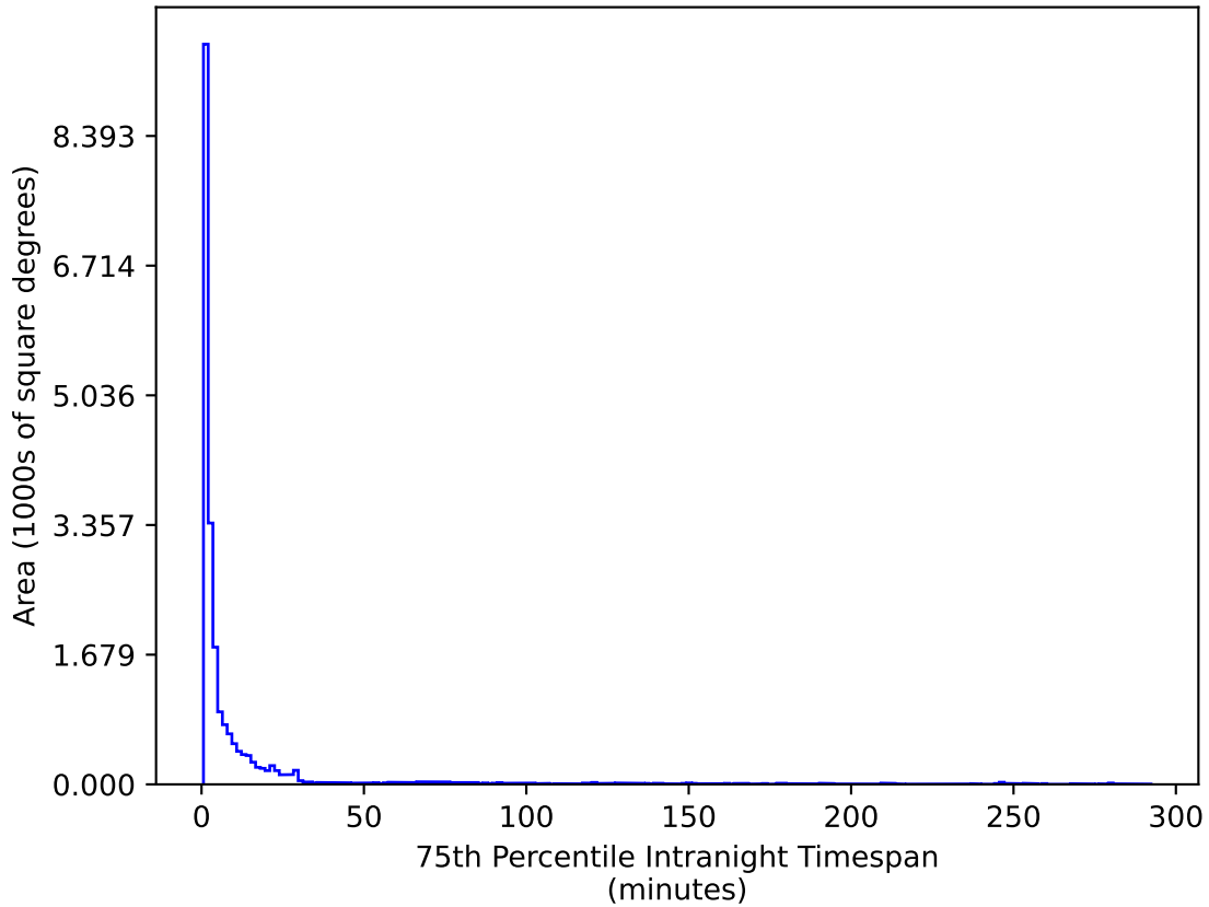
ddf_acor_sf10_ls15_lsr10_v3.4_10yrs All sky u band: 75th Percentile Intranight Timespan
