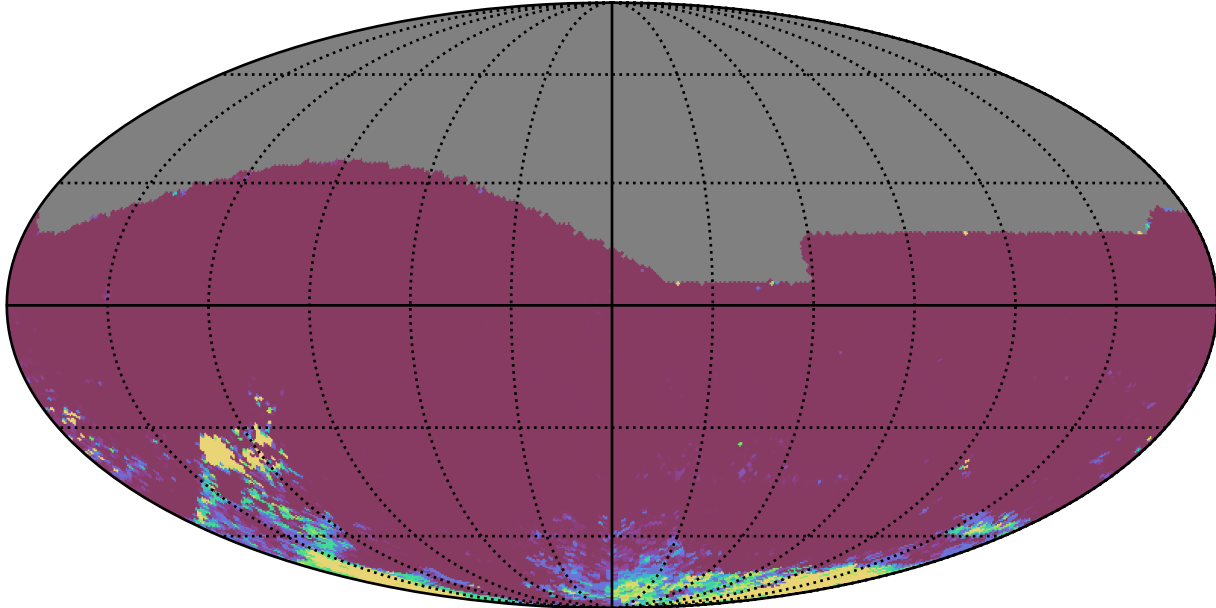
ddf_acor_sf10_lsf15_lsr10_v3.4_10yrs All sky ri bands: 75th Percentile Intranight Timespan
