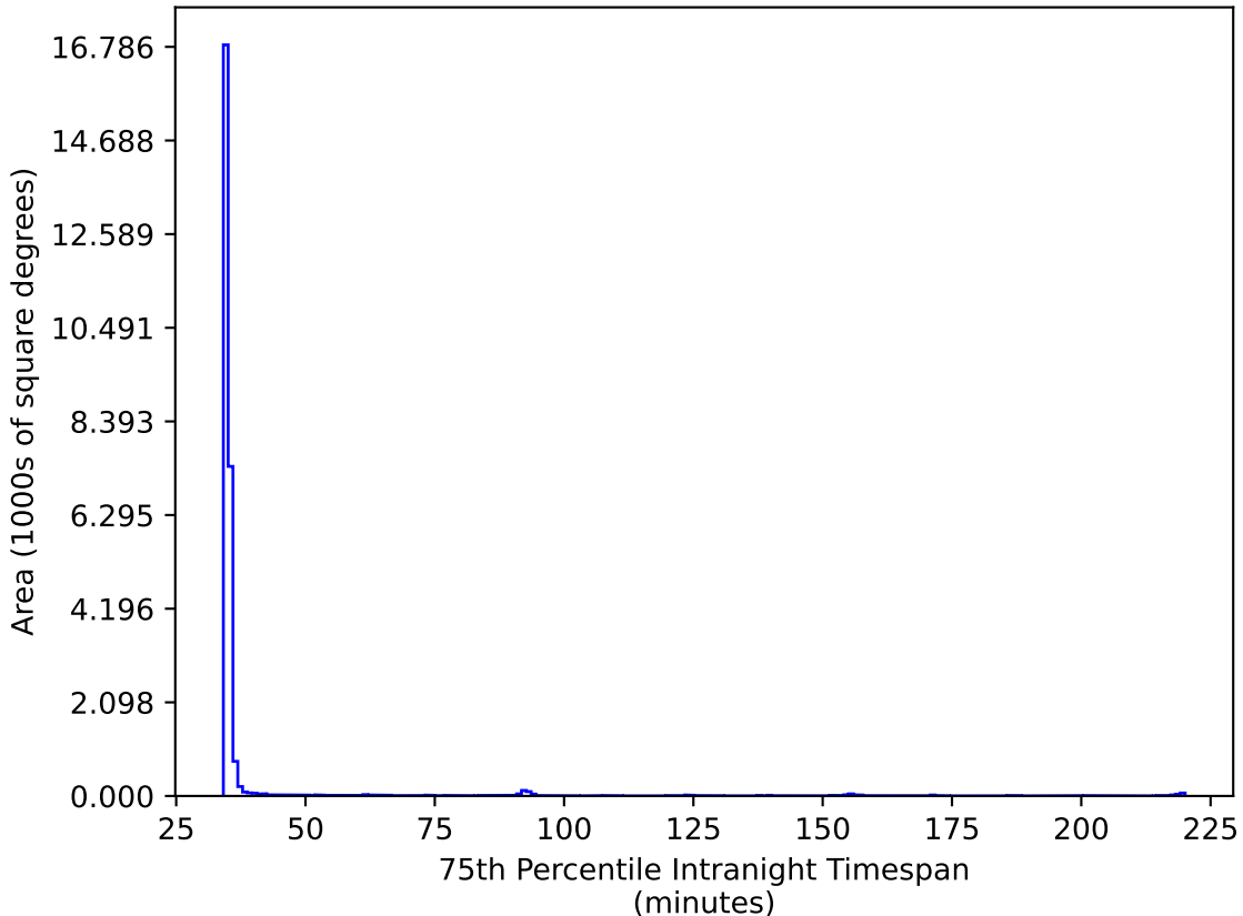
ddf_acor_sf10_lsf15_lsr10_v3.4_10yrs All sky ri bands: 75th Percentile Intranight Timespan
