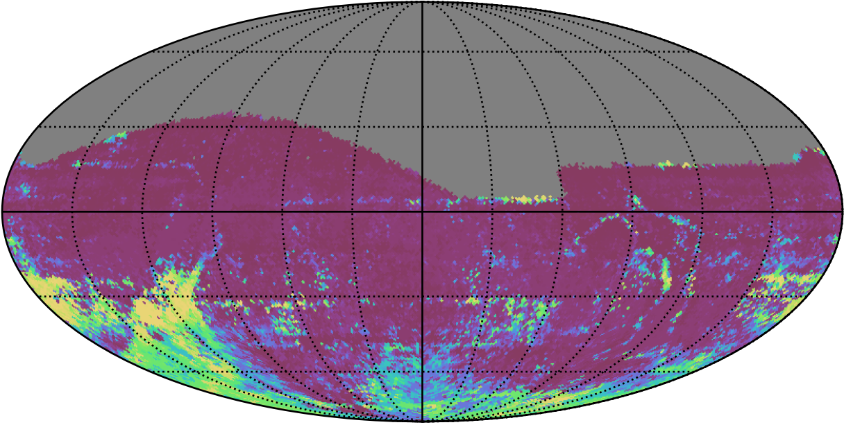
ddf_acor_sf10_lsf15_lsr10_v3.4_10yrs All sky r band: 75th Percentile Intranight Timespan
