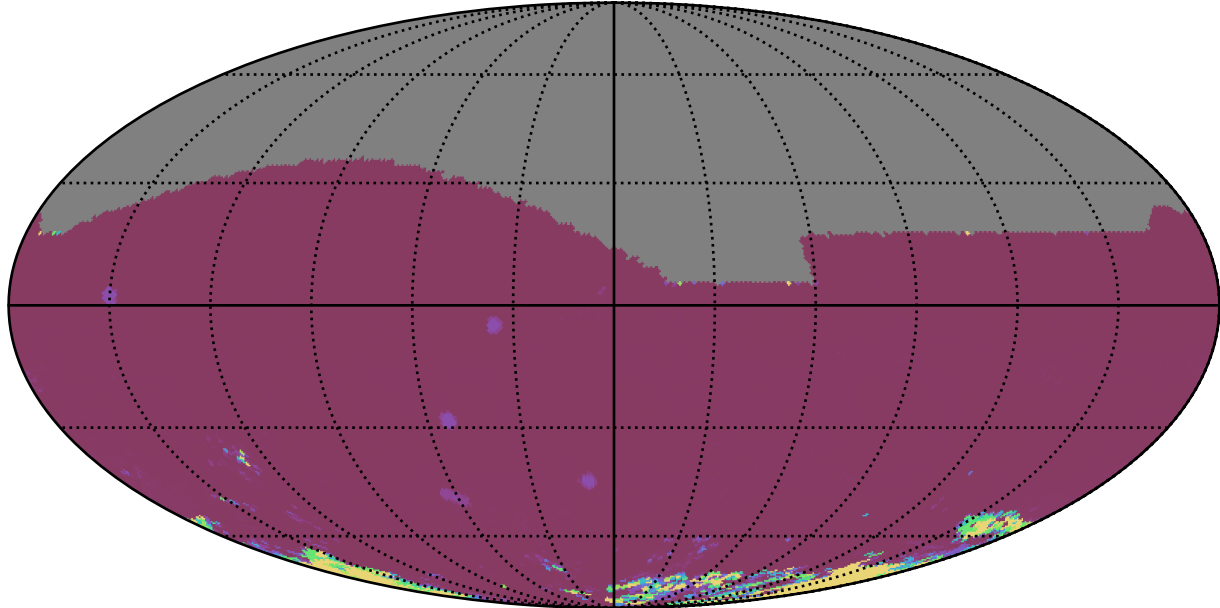
ddf_acor_sf10_lsf15_lsr10_v3.4_10yrs All sky iz bands: 75th Percentile Intranight Timespan
