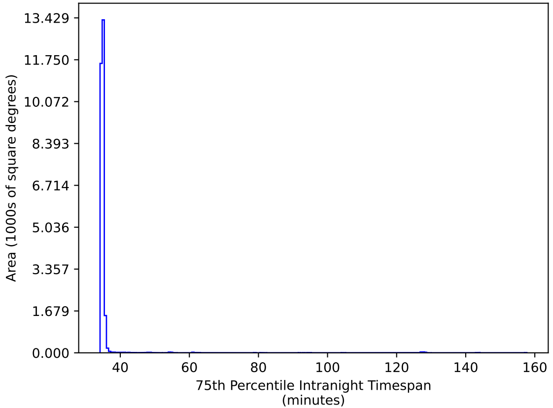
ddf_acor_sf10_lsf15_lsr10_v3.4_10yrs All sky iz bands: 75th Percentile Intranight Timespan
