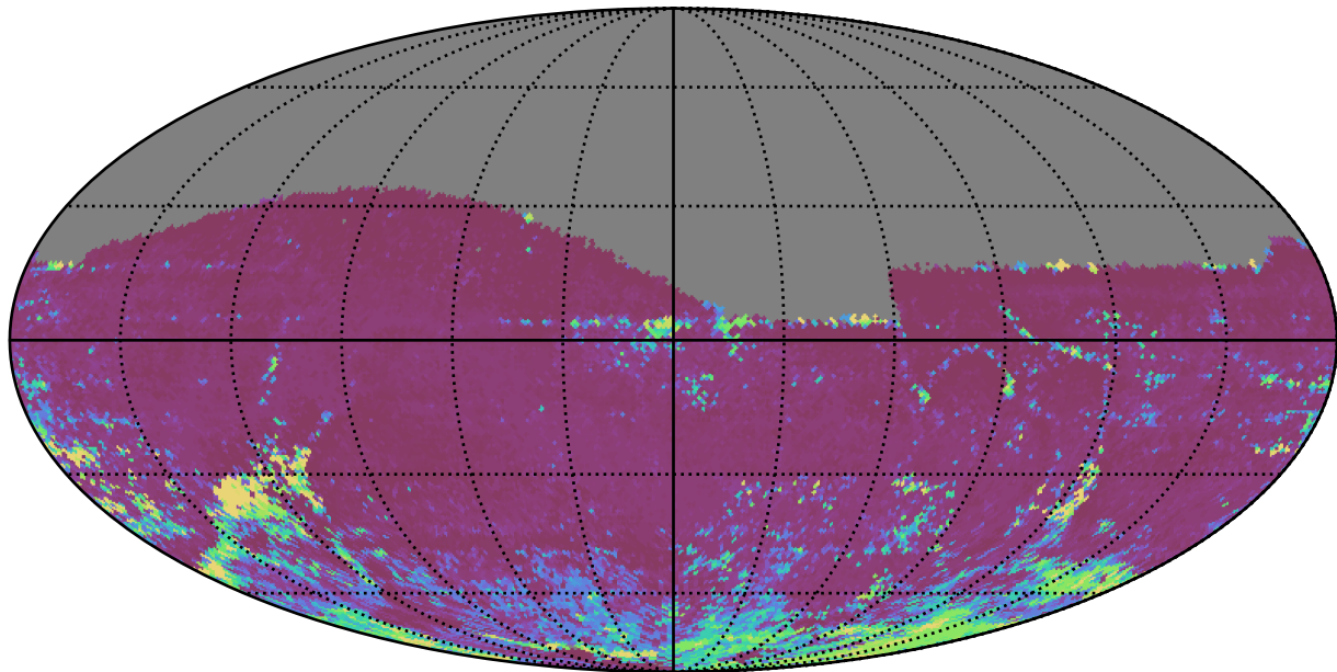
ddf_acor_sf10_ls15_lsr10_v3.4_10yrs All sky i band: 75th Percentile Intranight Timespan
