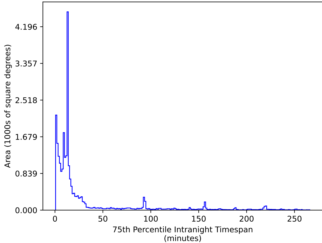
ddf_acor_sf10_lsf15_lsr10_v3.4_10yrs All sky i band: 75th Percentile Intranight Timespan
