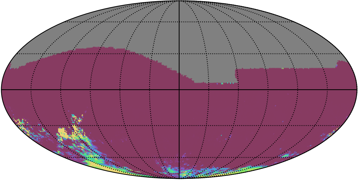
ddf_acor_sf10_lsf15_lsr10_v3.4_10yrs All sky gr bands: 75th Percentile Intranight Timespan
