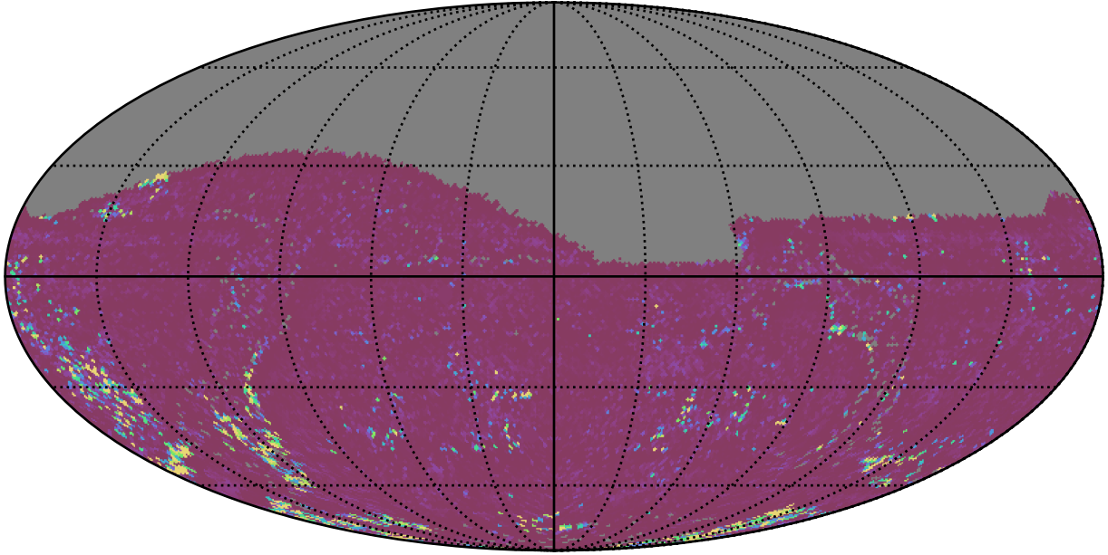
ddf_acor_sf10_lsf15_lsr10_v3.4_10yrs All sky g band: 75th Percentile Intranight Timespan
