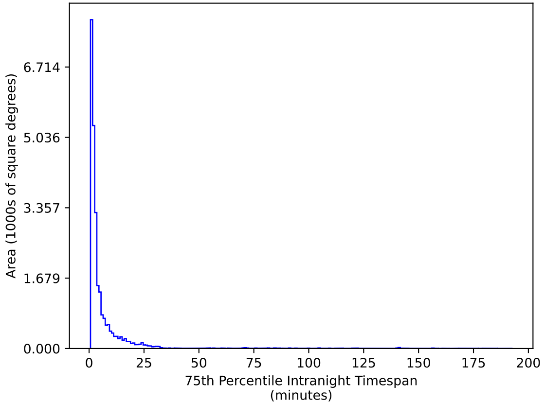
ddf_acor_sf10_lsf15_lsr10_v3.4_10yrs All sky g band: 75th Percentile Intranight Timespan
