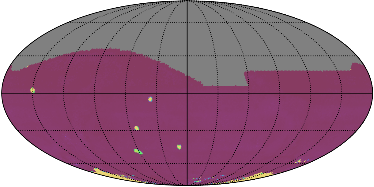
ddf_acor_sf10_lsf15_lsr10_v3.4_10yrs All sky all bands: 75th Percentile Intranight Timespan
