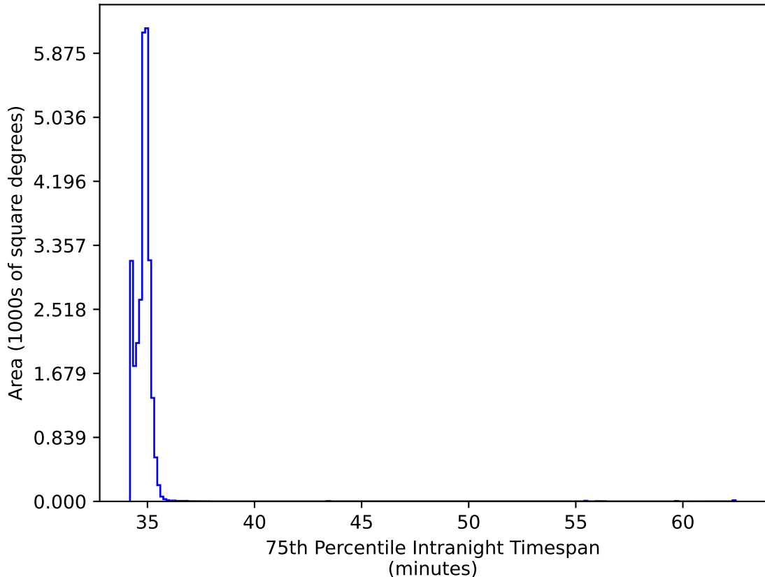
ddf_acor_sf10_lsf15_lsr10_v3.4_10yrs All sky all bands: 75th Percentile Intranight Timespan
