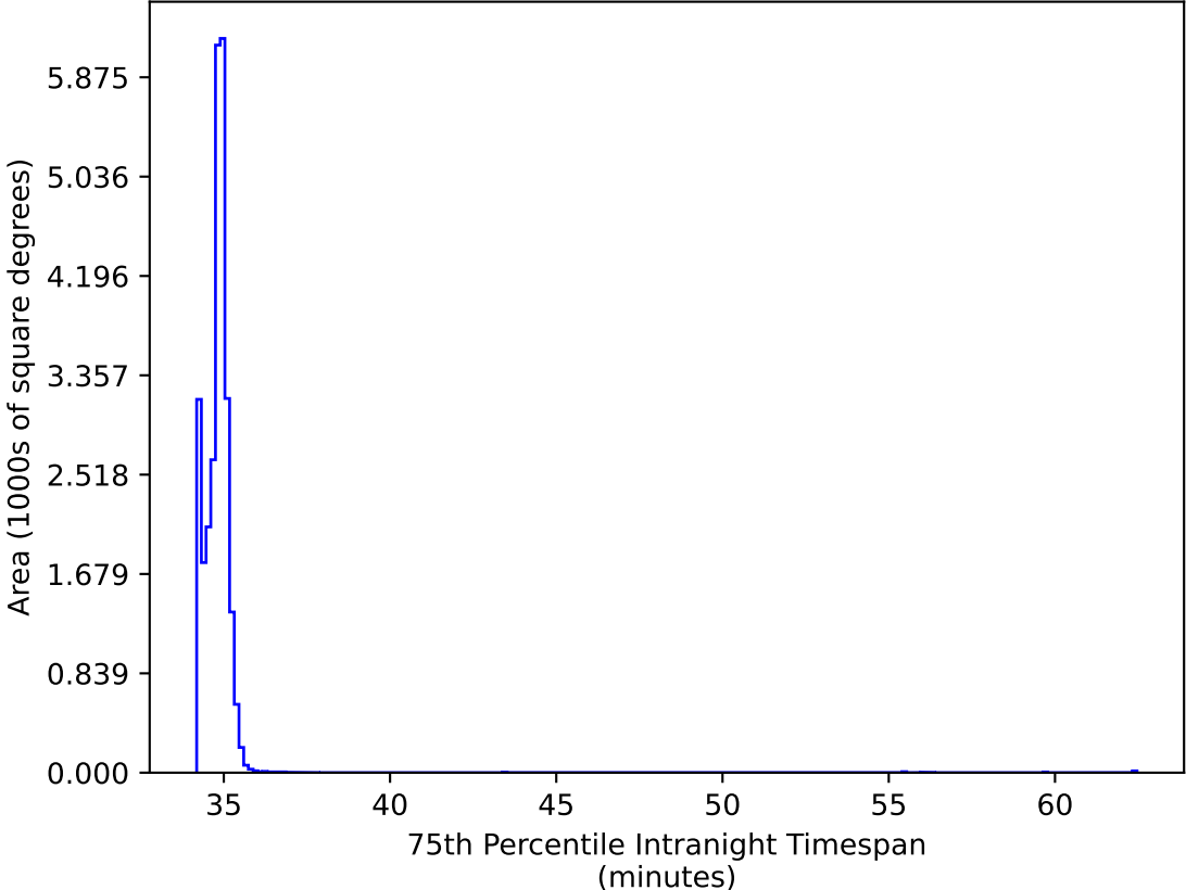
ddf_acor_sf10_lsf15_lsr10_v3.4_10yrs All sky: 75th Percentile Intranight Timespan
